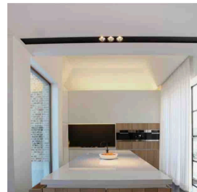
rails AND spots are recessed in the ceiling
